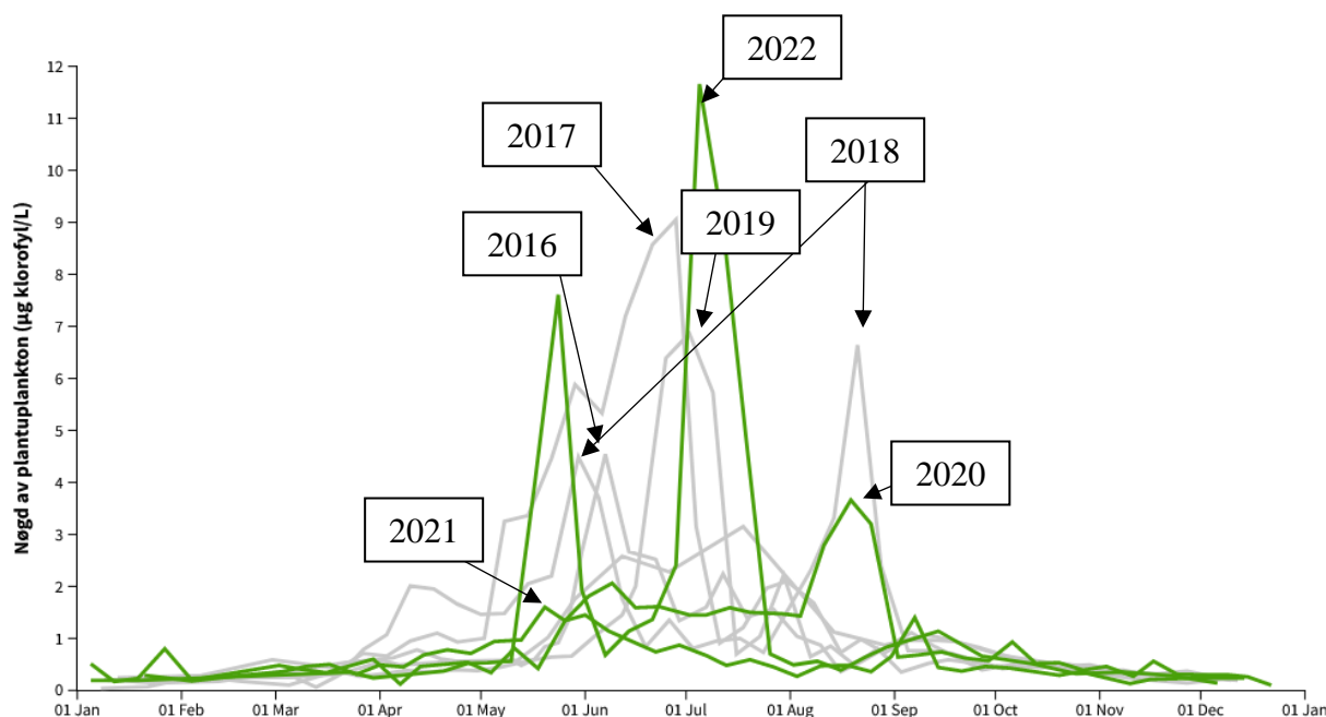
Figure 18. Chlorophyll a concentration on the Faroe shelf in the years from 2016 to 2022.
